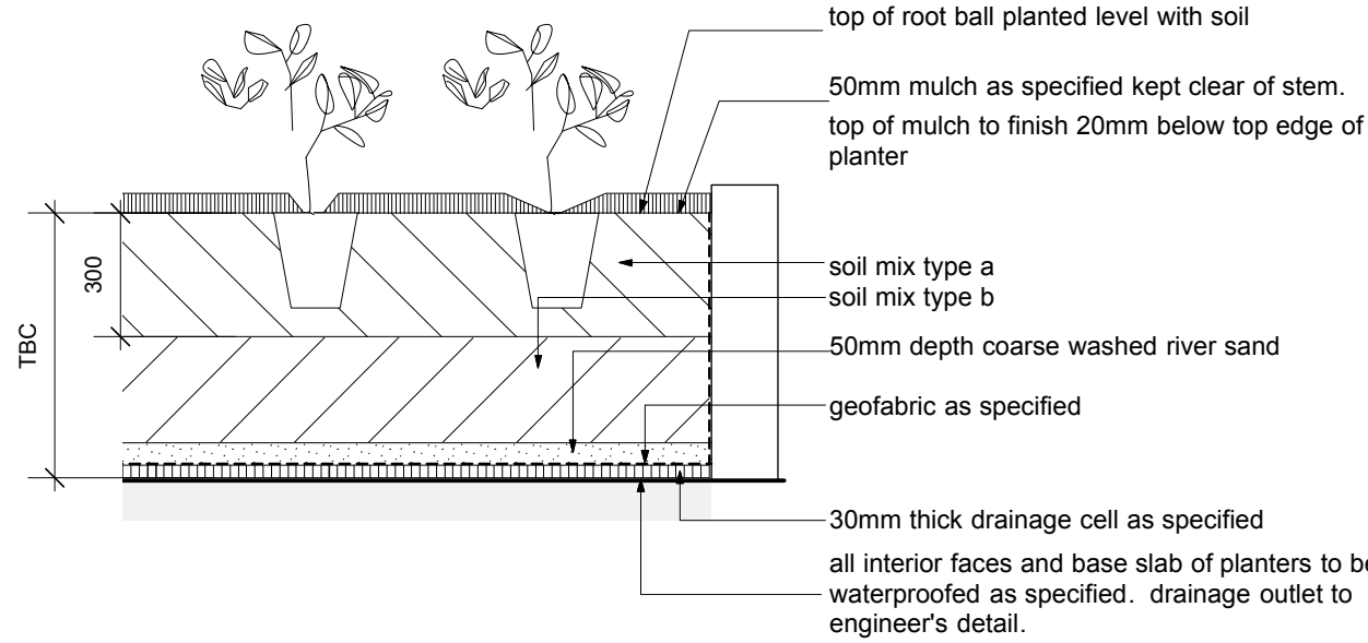
1 TYPICAL DETAIL - PLANTER BOX SCALE 1:20 @ A3
